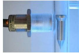
Inductive proximity switch (left) and float (right)
